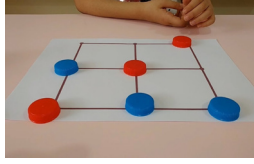
play tic-tac-toe
